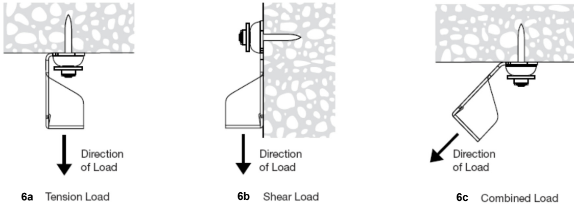
FIGURE 6—X-HS LOAD DIRECTIONS
