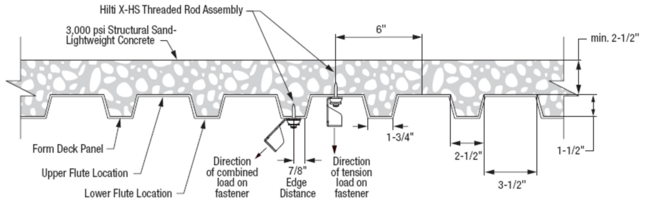
FIGURE 9—HILTI X-HS ROD HANGER ASSEMBLY LOCATION IN 1 1/2-INCH-DEEP FLOOR DECK PANEL, NORMAL DECK PANEL PROFILE ORIENTATION
