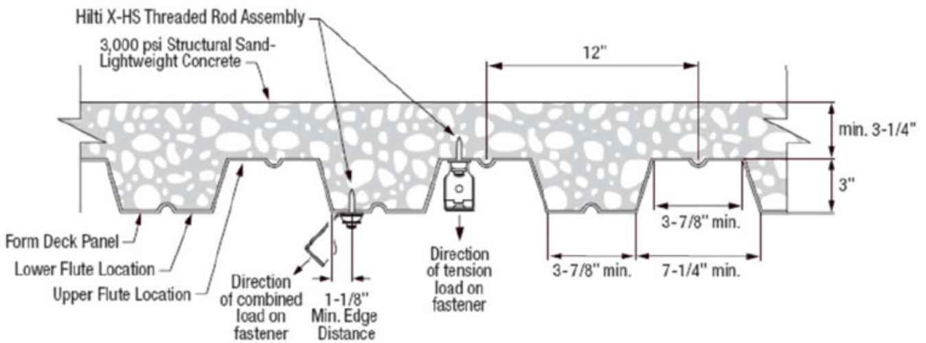
FIGURE 8—HILTI X-HS ROD HANGER ASSEMBLY LOCATION IN 3-INCH-DEEP COMPOSITE FLOOR DECK PANEL
